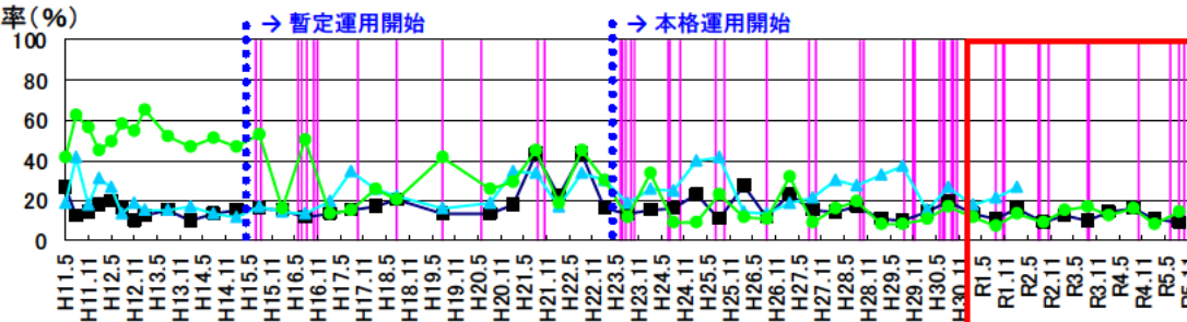
強熱減量(%)
